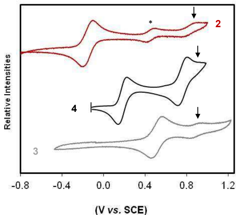
Fig. 2. Cyclic voltammogram of the zinc(II) porphyrins 2-4 in \text{CH}_2\text{Cl}_2/[\textit{n}\text{-Bu}_4\text{N}][\text{PF}_6] (0.1 M) at 25 °C at 0.1 V/s between -0.8 and 1.2 V vs. SCE, showing the Fe- (left) and Ru-centered (right) oxidations. The ZnTPP-based oxidations are indicated by an arrow, while the asterisk indicates the \text{FcH}/\text{FcH}^+ couple (0.46 V) used as an internal calibrant.
