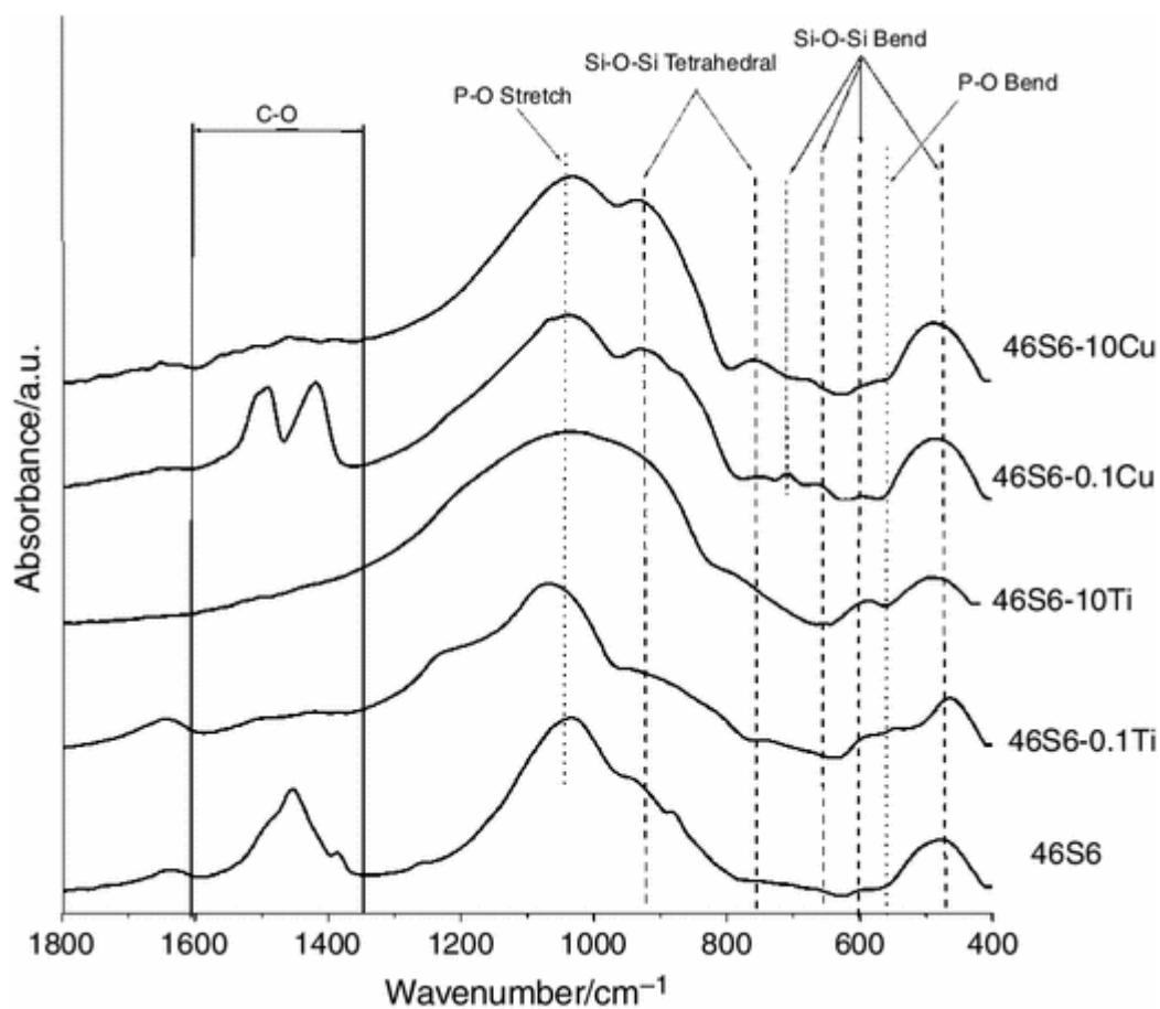
Fig. 2 FTIR spectra of pure and doped glasses
