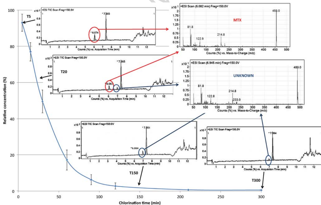
Fig. 6 – Behavior of MTX during chlorination in mass spectrometry. Relative concentration corresponds to the ratio C_0/C (obtained by fluorimetry after photooxidation); chromatograph peak at 7.4 min correspond to internal standard ( n = 2 ).
