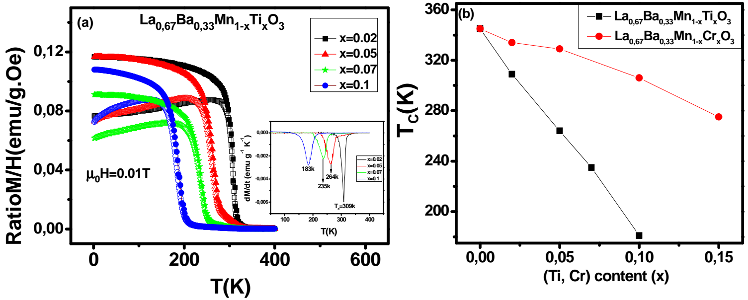
Figure 5: (a) Plots of the magnetization, measured in a field of 0.01T, versus temperature for Ti-substituted \text{La}_{0.67}\text{Ba}_{0.33}\text{Mn}_{1-x}\text{Ti}_x\text{O}_3 in field-cooled (filled symbols) and zero-field-cooled (open symbols) modes. Inset shows the temperature derivative dM/dT , (b) T_c versus (Ti, Cr) content x .
