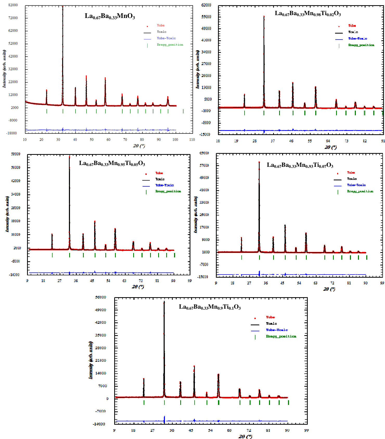
Figure 2 : Rietveld refinement of X-ray diffraction data for \text{La}_{0.67}\text{Ba}_{0.33}\text{Mn}_{1-x}\text{Ti}_x\text{O}_3 ( 0 \leq x \leq 0.1 ). Open circles correspond to the X-ray diffraction data and the lines are theoretical fits to the observed X-ray data. Vertical bars are the Bragg reflections for the space group \text{Pm}\bar{3}\text{m} . The difference pattern between the observed data and the theoretical fit is shown at the bottom.
