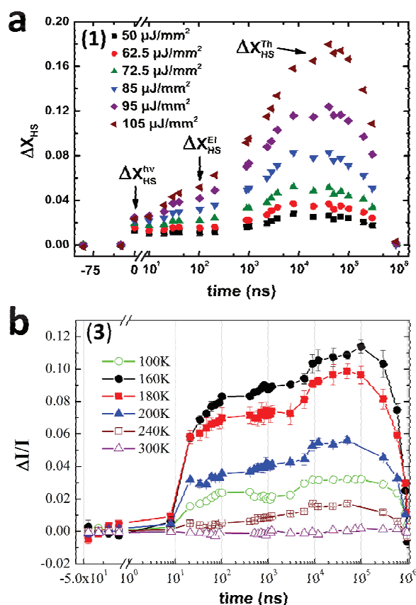
Fig.10.(a) Photo-excited fraction of HS molecules at 140K as a function of pump energy for (1) revealing the 3 steps of photoinduced ( \Delta X_{HS}^{hv} ), elastic ( \Delta X_{HS}^{El} ) and thermal ( \Delta X_{HS}^{Th} ) nature and (b) photo-response of (3) for different temperatures. Figures were partly reproduced from ref. [55], with permission of the copyright holders.
