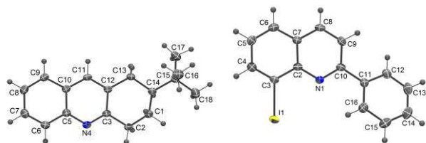
Figure 1 ORTEP diagram (50% probability) of 1e and 2a .
