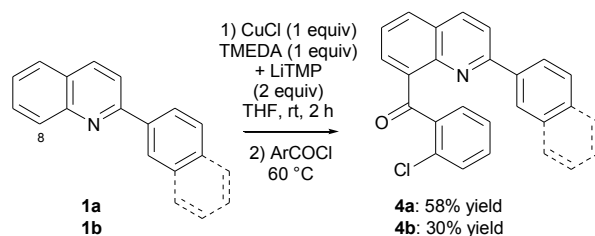
Scheme 8 Deproto-metallation of 1a,b followed by aroylation.
