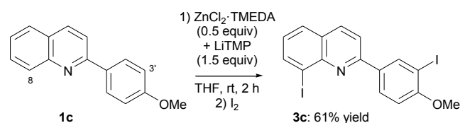
Scheme 3 Deprotonation of 1c followed by iodination.
