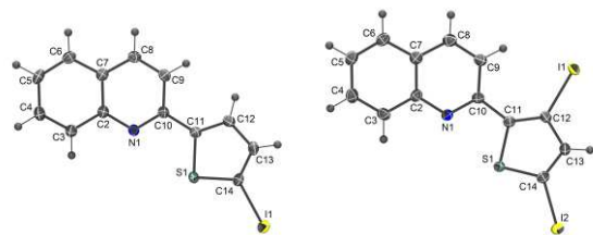
Figure 2 ORTEP diagrams (50% probability) of 2h and 3h .
