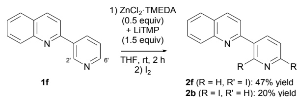
Scheme 5 Deprotonation of 1f followed by iodination.
