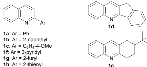
Scheme 1 Quinolines 1 for which the deproto-metallation was studied.
