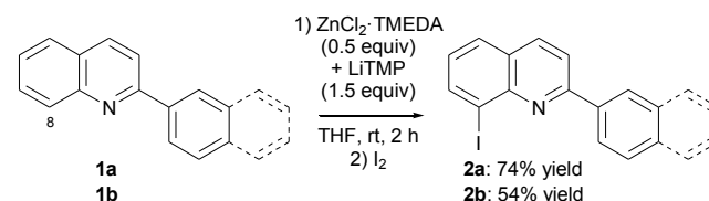
Scheme 2 Deprotonation of 1a,b followed by iodination.
