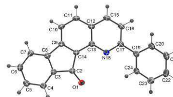
55 Figure 4 ORTEP diagrams (50% probability) of 5a .
