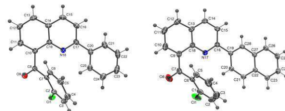
40 Figure 3 ORTEP diagrams (50% probability) of 4a and 4b .
