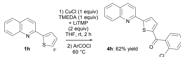
Scheme 9 Deproto-metallation of 1h followed by aroylation.
