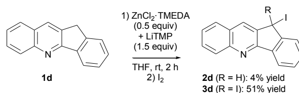
Scheme 4 Deprotonation of 1d followed by iodination.
