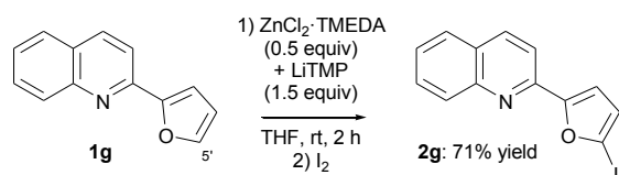
5 Scheme 6 Deproto-metallation of 1g followed by iodination.
