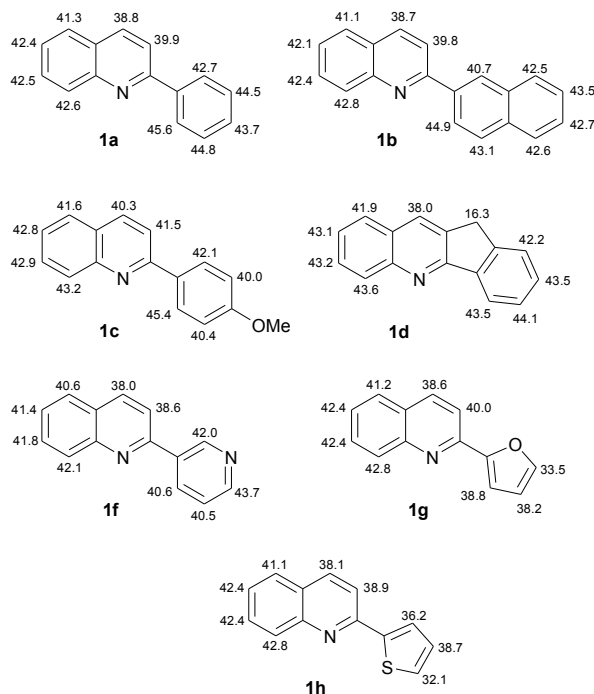
Scheme 11 Calculated values of pK_a(\text{THF}) of the quinoline substrates.
