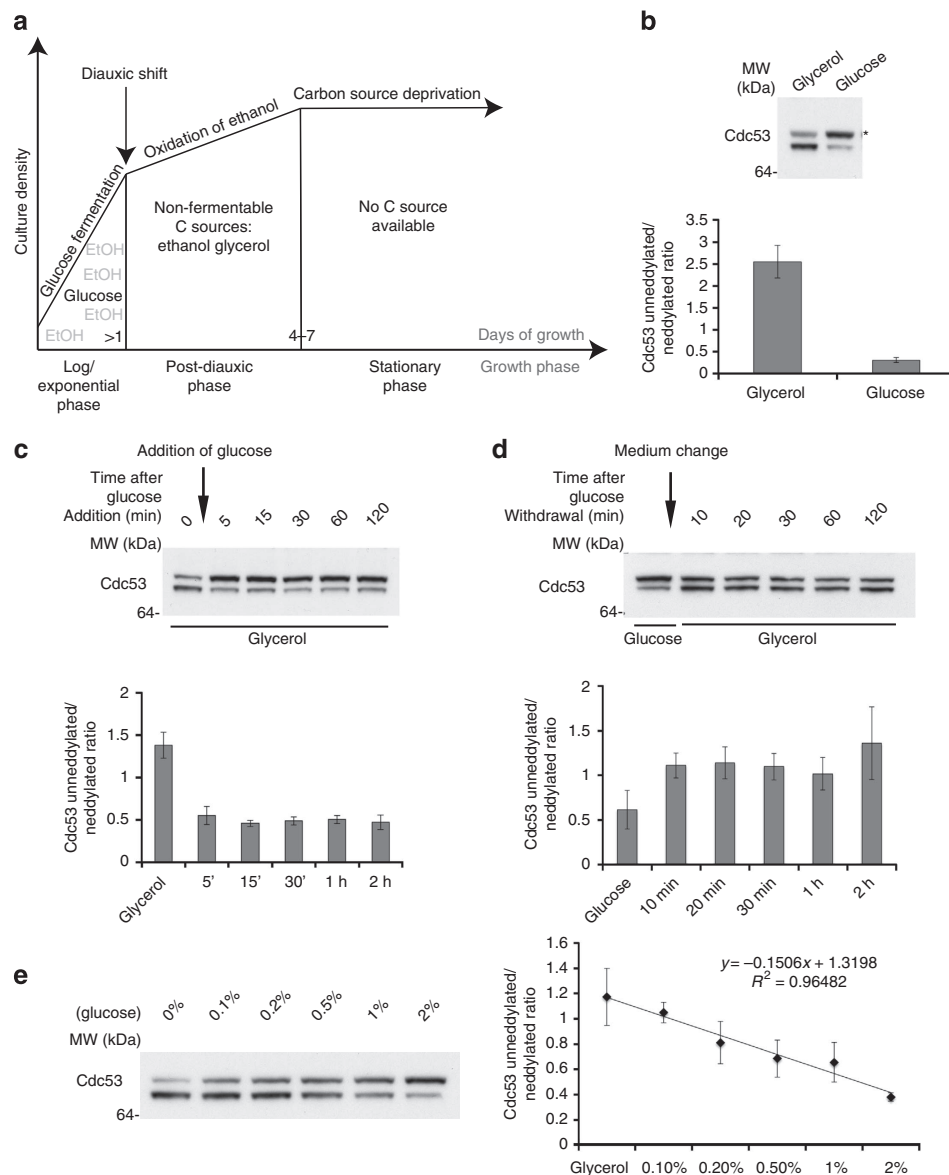
Figure 1 | The neddylation status of budding yeast Cdc53/Cul1 is sensitive to changes in carbon source. (a) Yeast carbon source utilization. Yeast ferment glucose during an exponential/log phase of growth and as a by-product, ethanol is released. Following glucose exhaustion, yeast switch from glucose fermentation to oxidative phosphorylation of non-fermentable carbon sources (for example, ethanol, glycerol). This metabolic switch is termed 'diauxic shift' and it marks an entry into a new phase of growth (post-diauxic phase). Complete exhaustion of carbon sources results in yeast entering stationary phase. (b) Yeast grown in glycerol-containing medium show markedly reduced neddylation of Cdc53/Cul1 as compared with cells grown on glucose. Asterisk indicates neddylated Cdc53/Cul1. Lower panel shows quantification as a mean of the ratio between unneddylated to neddylated Cdc53/Cul1. Error bars indicate s.d. ( n = 3 ). (c) Glucose was added to yeast grown in glycerol media, and the changes in neddylation were chased over time. Cdc53/Cul1 is fully neddylated already 5 min after glucose addition (quantification below as in Fig. 1a; error bars indicate s.d. ( n = 3 )). (d) Cells were grown in glucose-containing medium, pelleted, washed and resuspended in medium containing glycerol as sole carbon source. Neddylation of Cdc53/Cul1 was monitored over time. Change from glucose to glycerol medium induces a rapid reduction in Cdc53/Cul1 neddylation (quantification below as in Fig. 1a; error bars indicate s.d. ( n = 3 )). (e) Cells were grown in a medium containing the indicated concentration of glucose as sole carbon source. Cdc53/Cul1 neddylation increases linearly with the glucose concentration in the medium (quantification to the right; error bars indicate s.d. ( n = 3 )).
