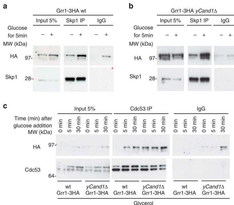
Figure 7 | yCand1 is required for the association of Skp1-Grr1 to the cullin-RING core after glucose addition. Skp1 immunoprecipitations (IPs) from wild-type (WT; a ) or yCand1-deleted cells ( b ) carrying endogenously tagged Grr1-3HA. In glycerol, low amounts of Grr1-3HA are associated with Skp1 in both strains. Within 5 min of glucose stimulation, an increase in Grr1-3HA bound to Skp1 is apparent in both WT and yCand1Δ cells. ( c ) Cdc53/Cul1 IPs from WT or yCand1-deleted cells carrying endogenously tagged Grr1-3HA. In WT cells, Grr1-3HA does not coimmunoprecipitate with Cdc53/Cul1 in glycerol medium. Five minutes upon glucose stimulation an interaction between Grr1-3HA and Cdc53/Cul1 is detectable, and this interaction is also maintained 30 min after glucose addition. In cells devoid of yCand1, Grr1-3HA association with Cdc53/Cul1 is detectable even in glycerol media, but there is no increase in association 5 min after glucose addition. A slight increase is detectable 30 min after glucose was supplied to the cells.
