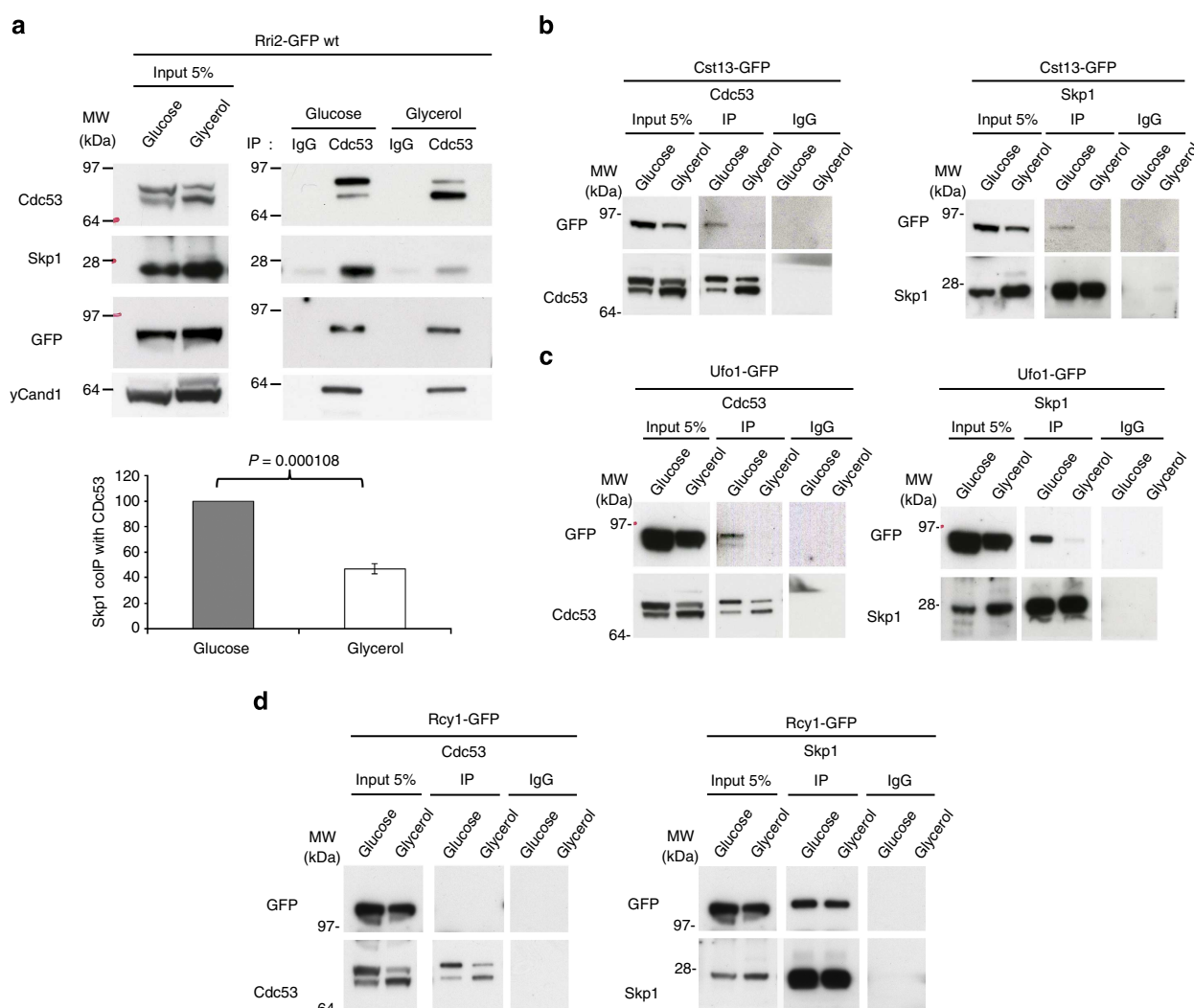
Figure 3 | Substrate adaptor/receptor modules dissociate from Cdc53/Cul1 and Skp1 during inactivation of the SCF. (a) Immunoprecipitation (IP) of Cdc53/Cul1 from cells grown in glucose or glycerol. There is no difference in the amount of coimmunoprecipitated yCand1 or Rri2-GFP (CSN subunit), while a significant loss of Skp1 substrate adaptor is detectable in glycerol. Quantification of the Skp1 signal below. Error bars indicate s.d. ( n = 4 ; P = 0.000108 was calculated using Student's two-tailed t -test). (b) Cdc53/Cul1 (left panel) and Skp1 (right panel) IP from glucose- or glycerol-grown yeast. Endogenously tagged Cst13-GFP association with Cdc53/Cul1 and Skp1 is significantly reduced in the presence of glycerol. (c) IP as in b, but from endogenously Ufo1-GFP-tagged strain. Growth on glycerol results in dissociation of Ufo1-GFP from Cdc53/Cul1 and Skp1, as assessed by its coimmunoprecipitation. (d) IP as in b, but from endogenously Rcy1-GFP-tagged strain. Rcy1 is an F-box protein that associates with Skp1 (right), but not Cdc53/Cul1 (left). For this non-SCF F-box protein interaction with Skp1, as assessed by its coimmunoprecipitation, is not affected by a change of carbon source.
