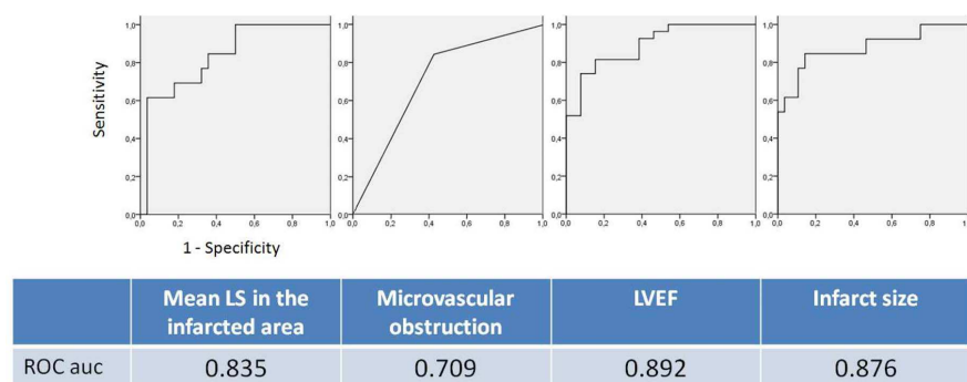
Figure 5. Nonparametric ROC plots of several imaging baseline parameters to the presence of a 3 segment akinesia at follow-up. doi:10.1371/journal.pone.0086959.g005
