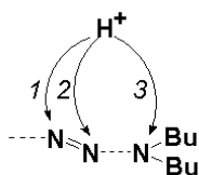
Scheme 2. The three possible protonation sites of 2a . 1 corresponds to the protonation at N(39); 2: N(40); 3: N(48).
