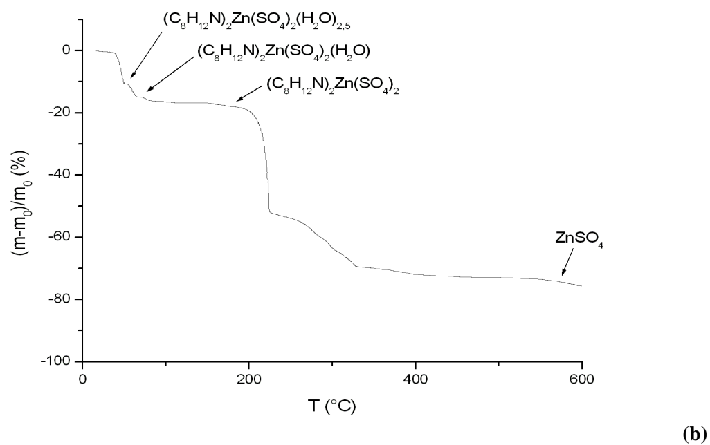
Figure 5: TG curve for the decomposition of (C_8H_{12}N)_2[M(SO_4)_2(H_2O)_4](H_2O)_2 in air, for (a) Ni and (b) Zn.
