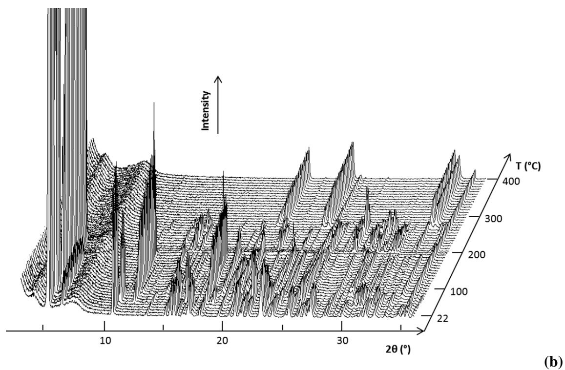
Figure 6: TDXD plot for the decomposition of the compounds in air, showing the successive crystalline phases up to \text{MSO}_4 , for (a) Ni and (b) Zn.
