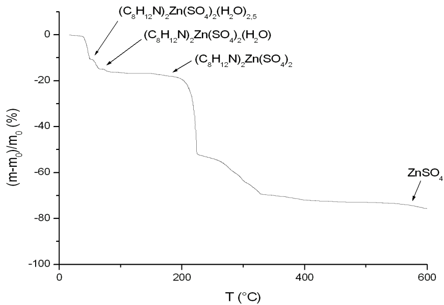
Figure 5: TG curve for the decomposition of (\text{C}_8\text{H}_{12}\text{N})_2[\text{M}(\text{SO}_4)_2(\text{H}_2\text{O})_4](\text{H}_2\text{O})_2 in air, for (a) Ni and (b) Zn.
