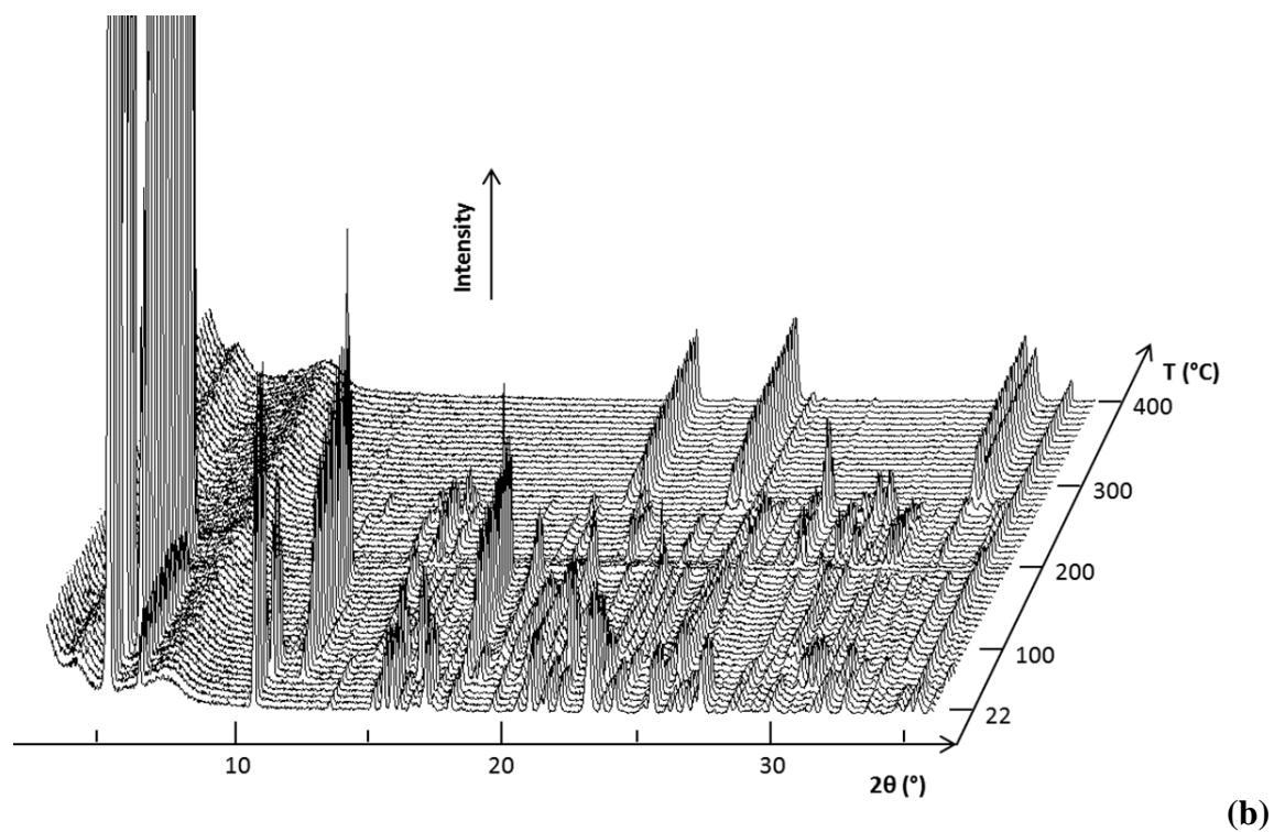
Figure 6: TDXD plot for the decomposition of the compounds in air, showing the successive crystalline phases up to \text{MSO}_4 , for (a) Ni and (b) Zn.
