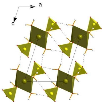
Figure 3: The weak hydrogen bonding between the [M^{II}(H_2O)_4(SO_4)_2]^{2-} entities within the mineral layer, showing its supramolecular aspect.
