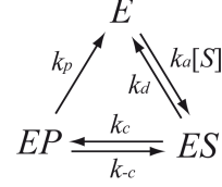
Figure 8. The first order cycle of the reaction of Fig.7, whose drawing is a prerequisite for using the King and Altman procedure.
