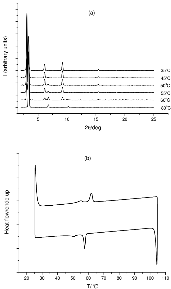
Figure 5. Powder X-ray diffractogram of complex 2b recorded at various temperature on cooling from isotropic liquid (a) and DSC trace (second heating – cooling cycle) of complex 2c (b).
