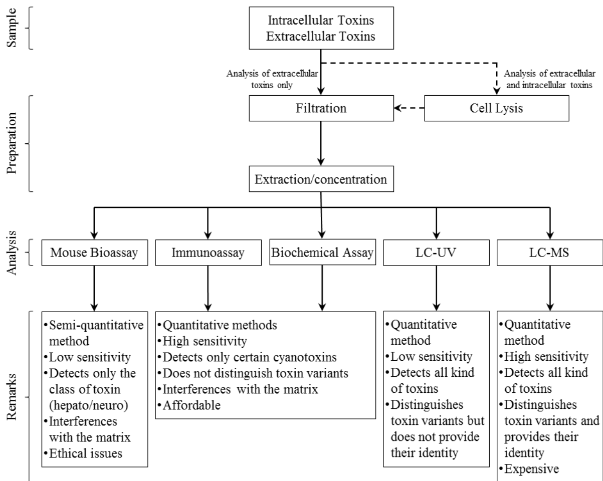
Fig. 5: Overview of sample preparation and analytical methods for the detection of cyanotoxins.
