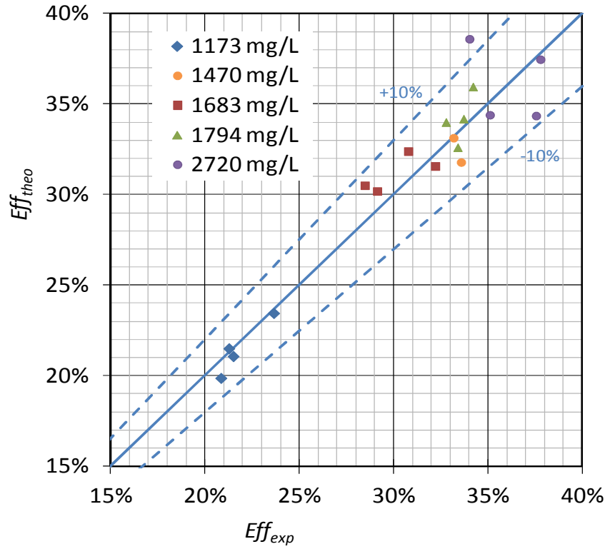
Figure 2: Parity diagram comparing the experimental values of the ozone removal efficiency with the theoretical values obtained with \alpha^\circ = 76.1 \text{ m}^2 \text{ m}^{-3} for various H_2O_2 concentrations.
