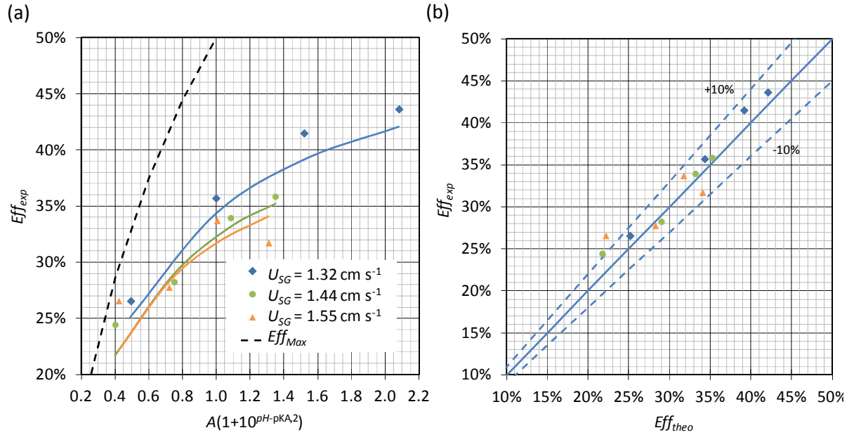
Figure 4: (a). \text{H}_2\text{S} removal efficiency vs. A(1+10^{\text{pH}-\text{pK}_{A,2}}) for various gas flow rates without chlorine. The colored lines represent the prediction of the model (Eq. 30) and the black line represents the prediction of the maximal removal efficiency (Eq. 29). (b). Parity plot between the experimental and predicted removal efficiencies.
