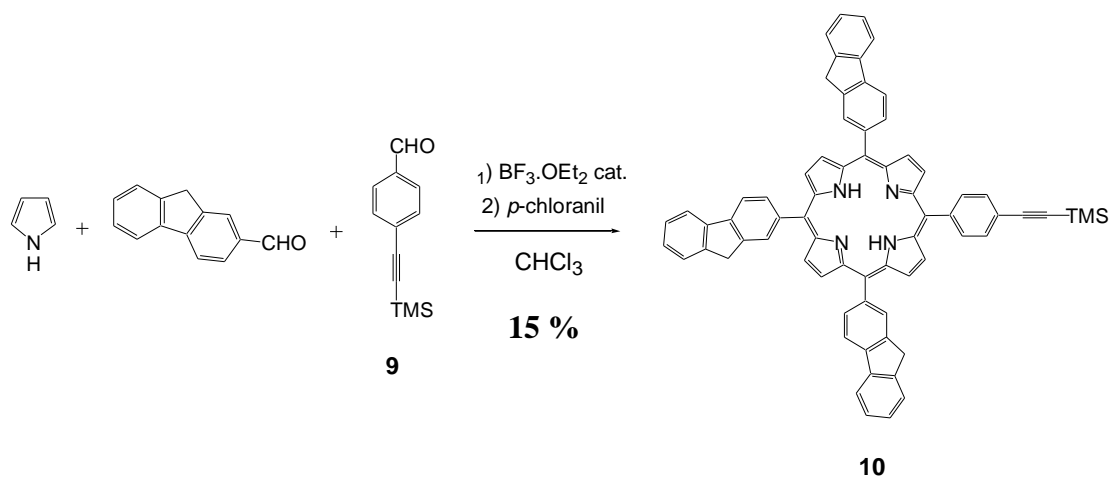
Scheme 2: Synthesis of porphyrin 10
