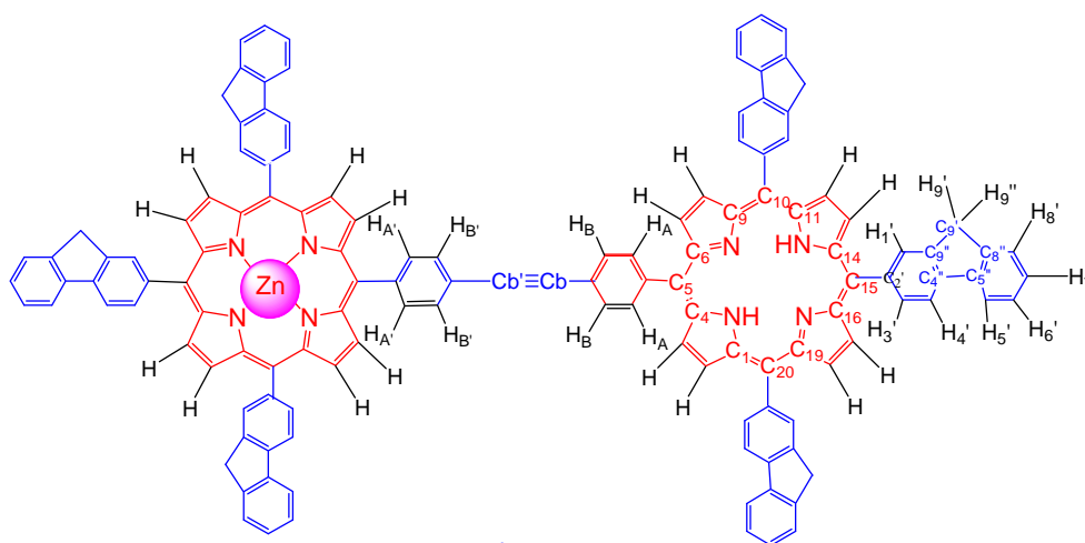
Figure 3: Hydrogen and carbon atom-labeling for new Dimer 7
