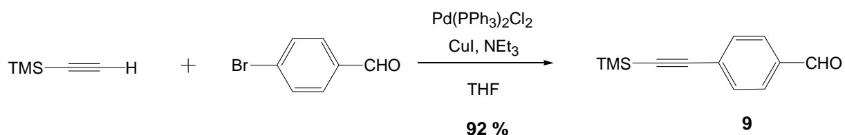
Scheme 1: Synthesis of compound 9 (4 - ((trimethylsilyl)ethynyl) benzaldehyde)
