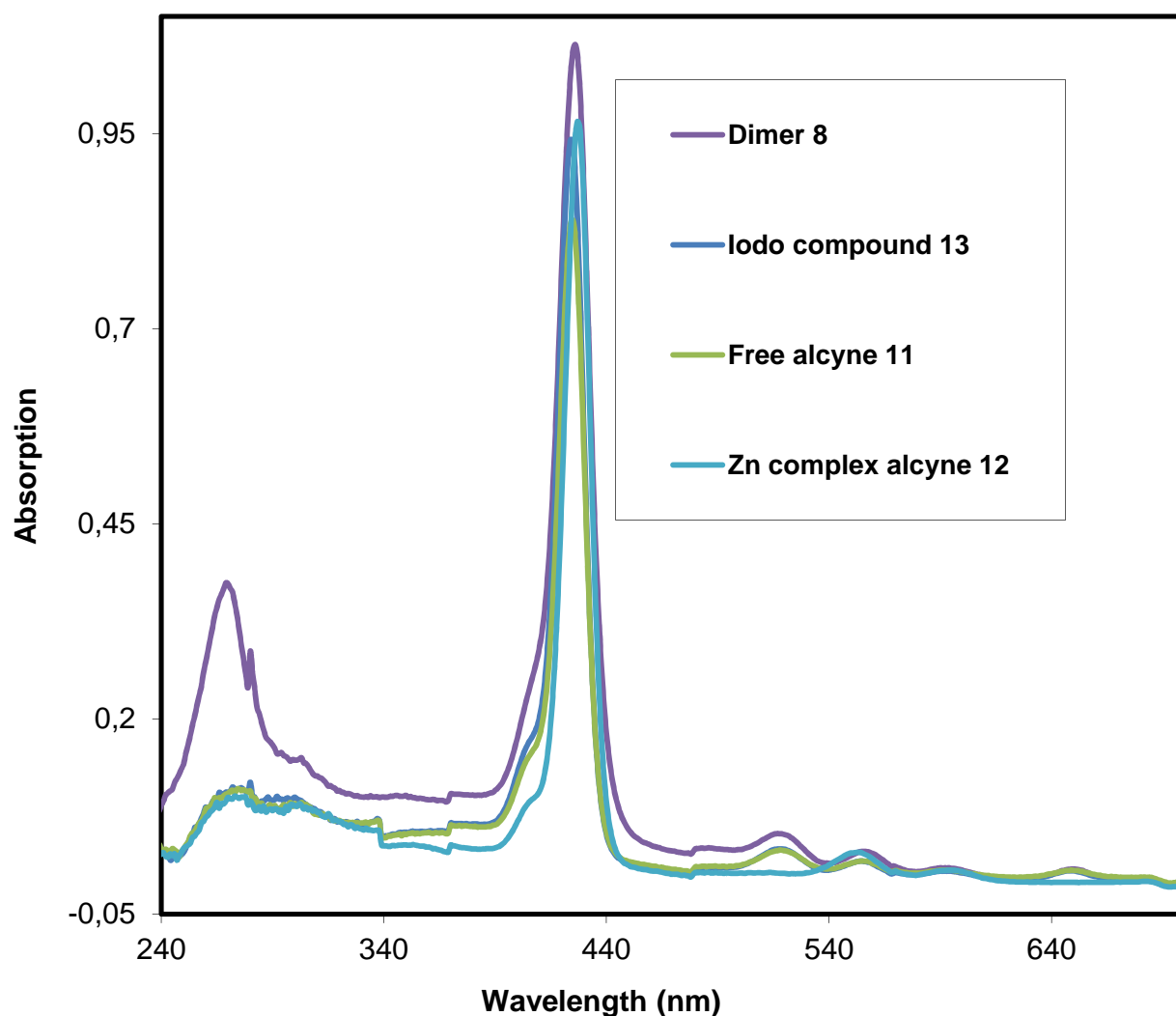
Figure 5: a/ Absorption spectra of TPP (red), TFP (pink), OOPF (dark blue), SOFP (green) and new dimers 7 (orange), 8 (violet) in DCM at room temperature. All the spectra are normalized to the spectrum of the reference TPP at 417 nm (concentration \sim 2.0 \cdot 10^{-6} M). b/ Formation of free dimer 8 by protonation of zinc complex 7 . c/ Absorption spectra of precursors 11 , 12 , 13 and new dimer 8 in DCM at room temperature.
