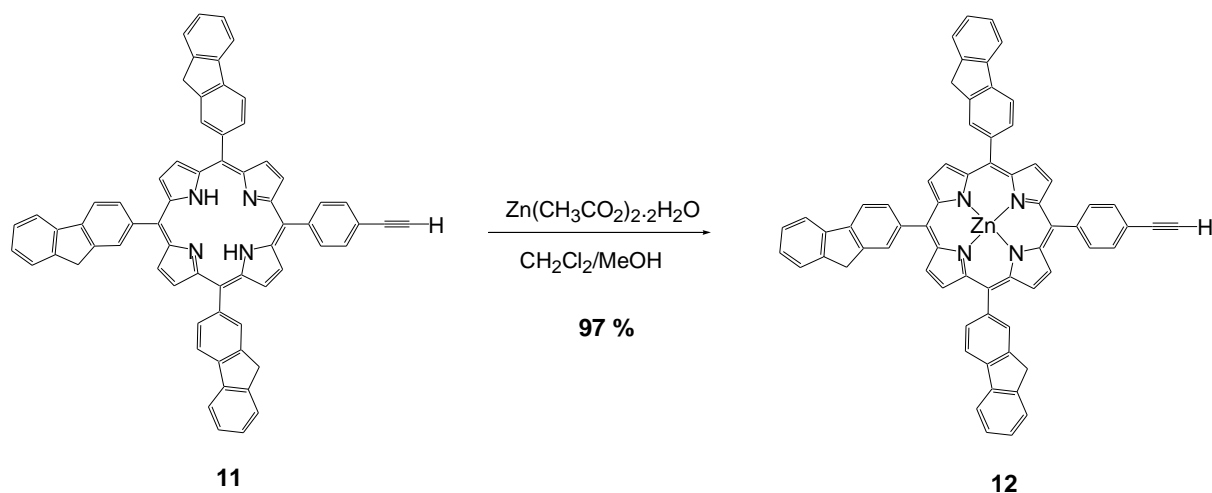
Scheme 4: Synthesis of zinc porphyrin complex 12
