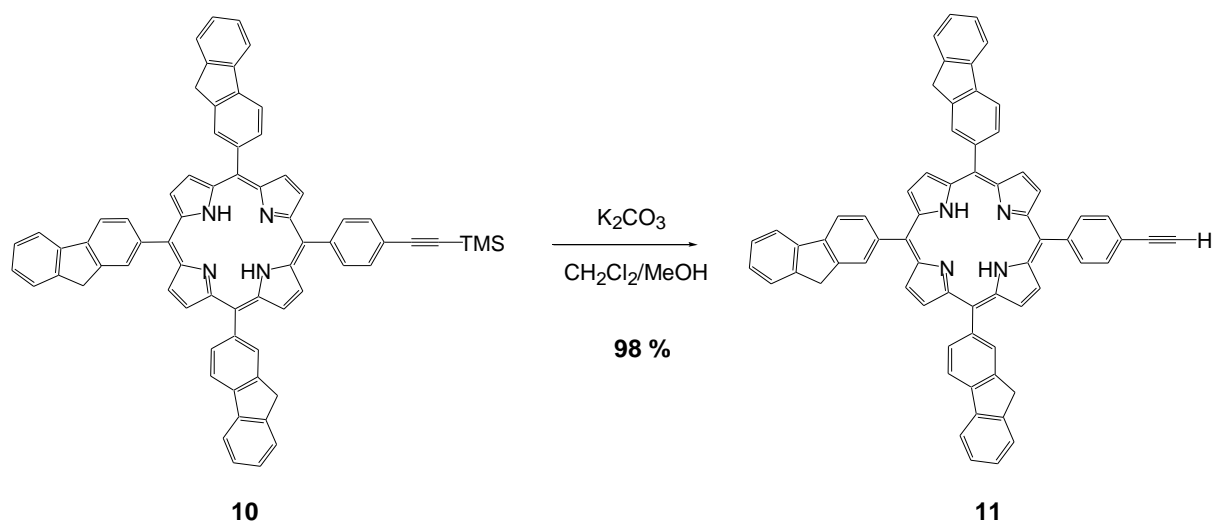
Scheme 3: Synthesis of porphyrin 11
