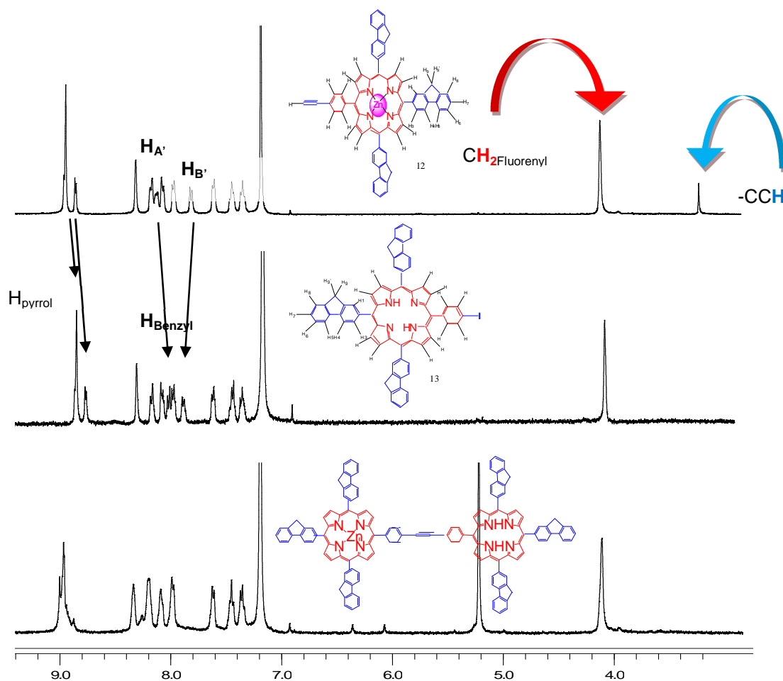
Figure 4: ^1\text{H-NMR} studies (in \text{CDCl}_3 ) of Dimer 7 (with a \text{CH}_2\text{Cl}_2 pic), in comparison to zinc porphyrin complex 12 (on the top) and for iodo porphyrin-intermediate 13 showing the shift as indicated by the arrows.
