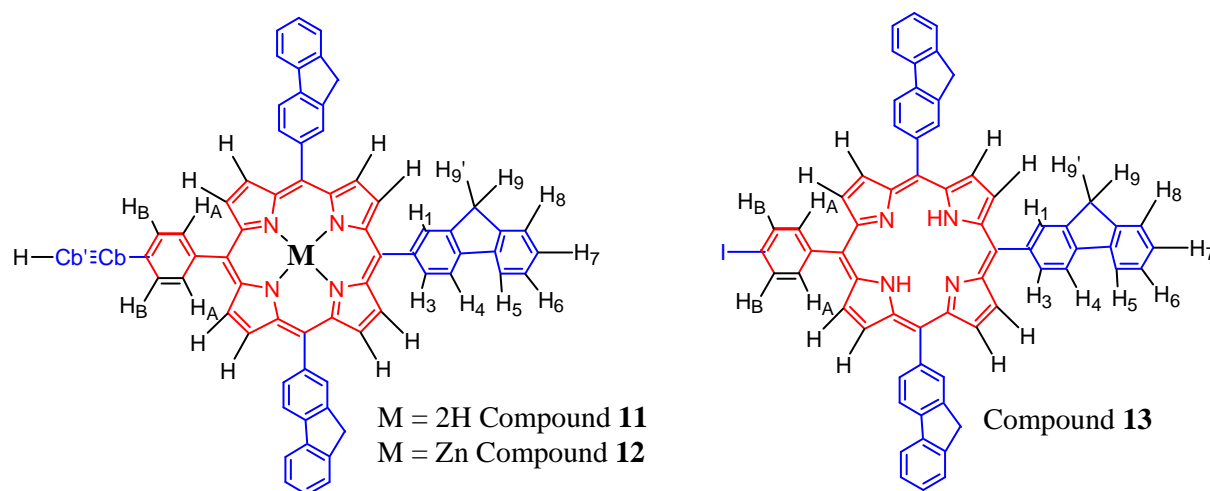
Figure 2: Hydrogen and carbon atom-labeling for porphyrins 11 , 12 and for iodo porphyrin-intermediate 13
