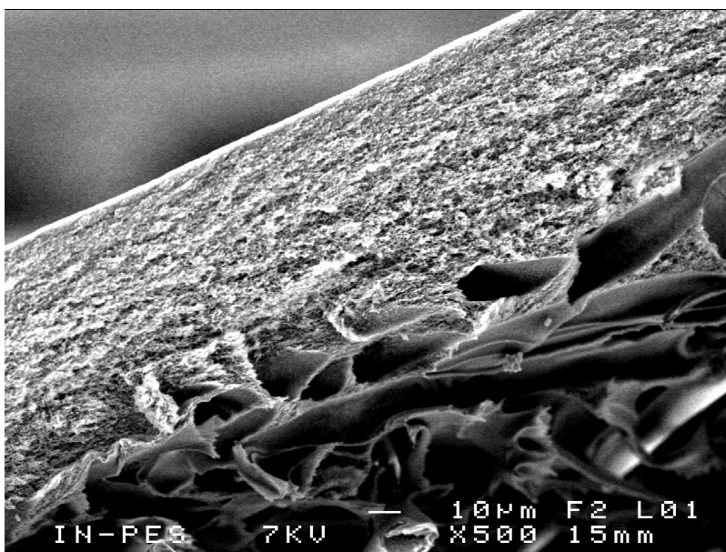
Fig. 2. SEM image of the cross-section of the HFK-131 composite membrane.
