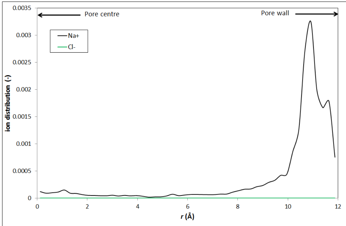
Figure 5. Radial distributions of \text{Na}^+ and \text{Cl}^- ions inside the deprotonated nanopore (bulk concentration: 1M).
