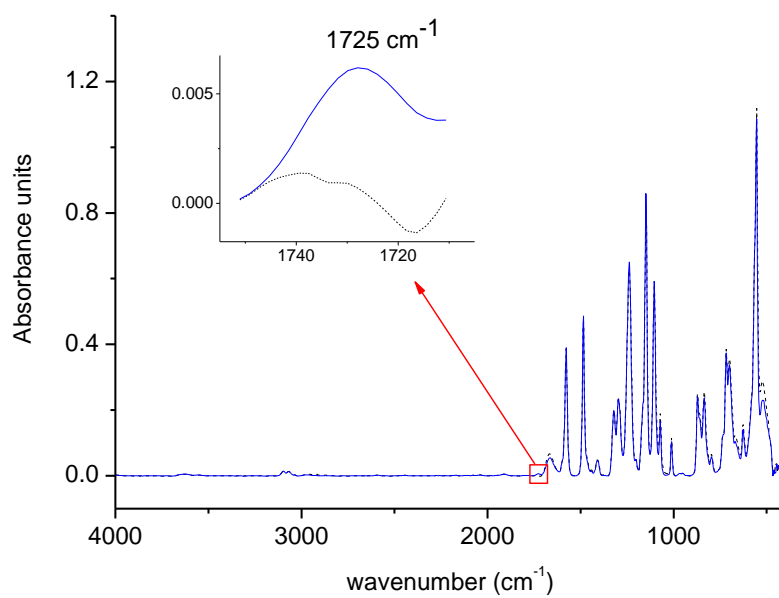
Figure 4: Representative ATR-FTIR spectra of PES membranes modified (blue solid lines) with solutions of with 3\text{-N}_2^+ (a), 2\text{-N}_2^+ (b) and 4\text{-N}_2^+ (c). Unmodified PES membrane spectra are also represented with black dashed lines. Blow-ups of the spectra are shown in insets.
