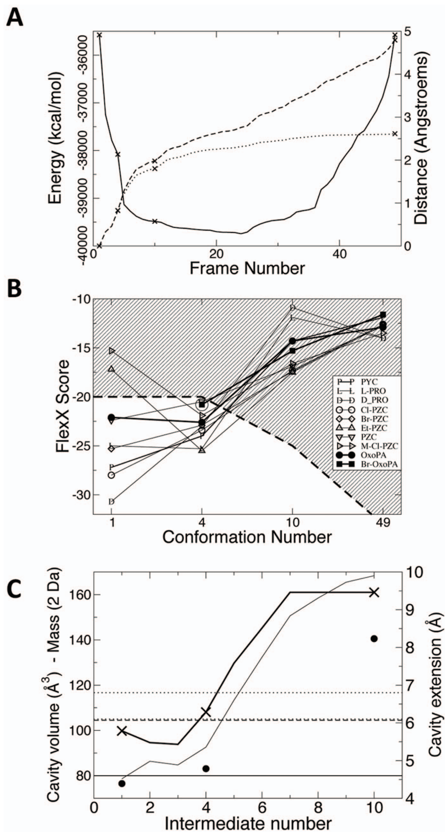
Figure 3. Transition path characteristics. (A) Energy profile and metric quantities for the TcPRAC transition path. The energy profile (full line) shows that the intermediate states have low energy and do not present any energy barriers. Dotted and dashed lines show the distance from the first structure ( d_{1,i} ) and the cumulative distance covered from the first structure ( l_{1,i} ), respectively (RMS in \text{\AA} , see Material and Methods). Little swerving was necessary to avoid the energy barriers. The points corresponding to the intermediate structures used in the screening are marked by crosses. (B) Scores of known ligands, synthesized analogues, and new inhibitors when docked in the selected binding site models. Br-OxoPA could not be docked
